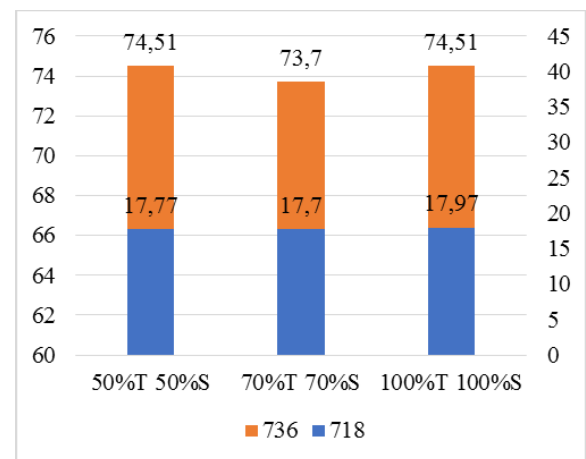
Fig. 13. Velocity [m/s] at 718 and 736 deg CA, cases 1, 2, 13.
