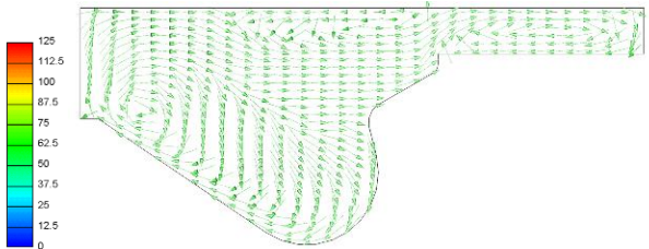
Fig. 8. Vertrices formation at 718 deg CA, case 10
