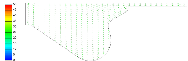
Fig. 3. Vortices formation at 718 deg CA, case 11
