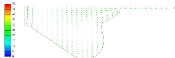
Fig. 4. Vortices formation at 718 deg CA, case 5
