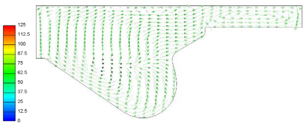
Fig. 9. Vertrices formation at 718 deg CA, case 5
