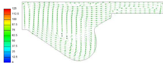
Fig. 12. Vertrices formation at 718 deg CA, case 13
